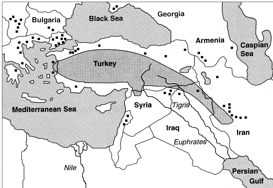
Fig. 1. Shaded area represents the main centre of origin of Triticum boeoticum , wild progenitor of T. monococcum ; dots indicate areas of secondary importance where T. boeoticum also has been found (from Harlan and Zohary 1966).
