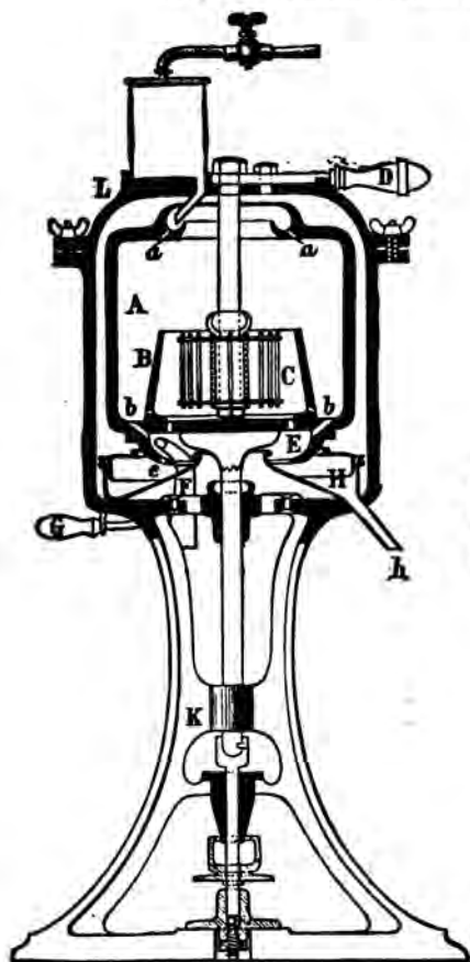
Fig. 2.— Swedish Cream Separator and Butter Extractor.
