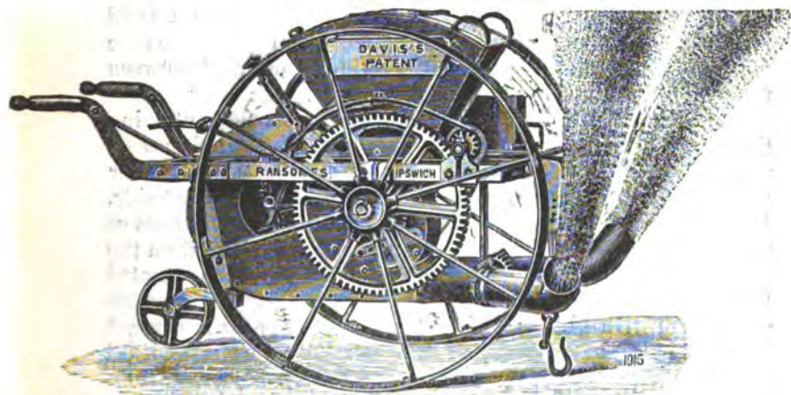
Fig. 24.—Sulphurator.
