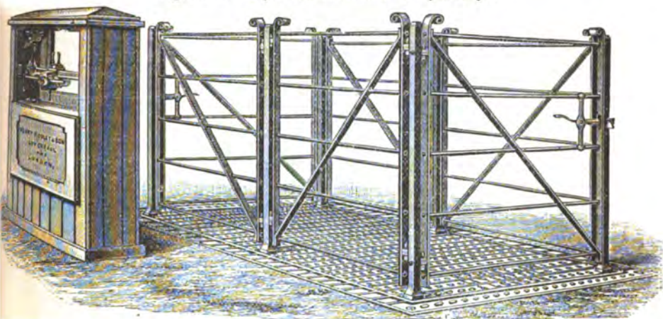
Fig. 7.—Pooley's Self-contained Weighbridge.
