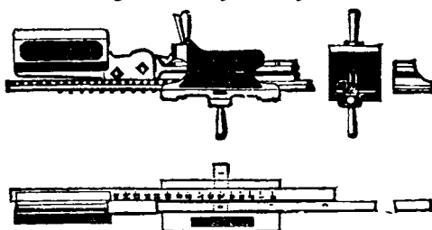
Fig. 6.—Avery's Steelyard.
