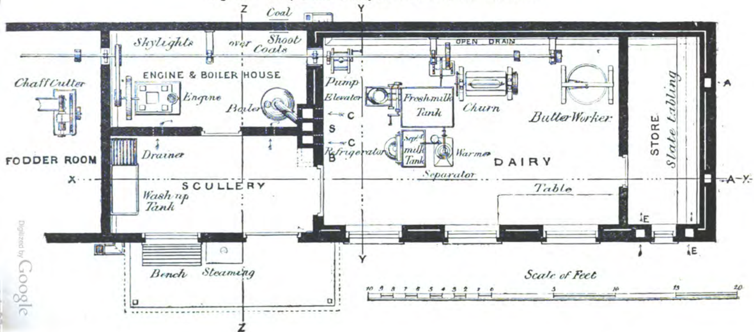
Fig. 1.—Plan of Butter Dairy for a Farm of over 100 Acres.
