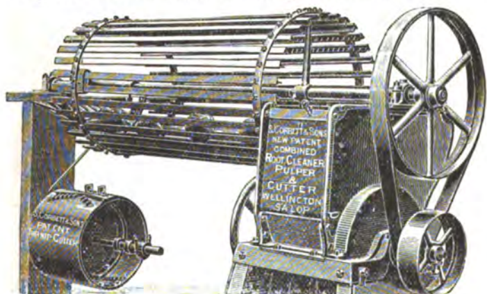
Fig. 10.—Corbett's Combined Turnip Cleaner and Slicer.
