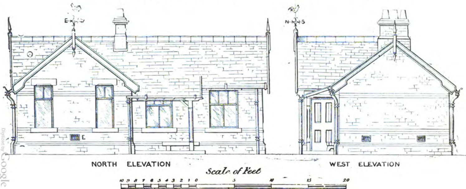
Figs. 7 and 8.— Butter Dairy for a Farm of under 100 Acres—North (Fig. 7) and West (Fig. 8) Elevations.
