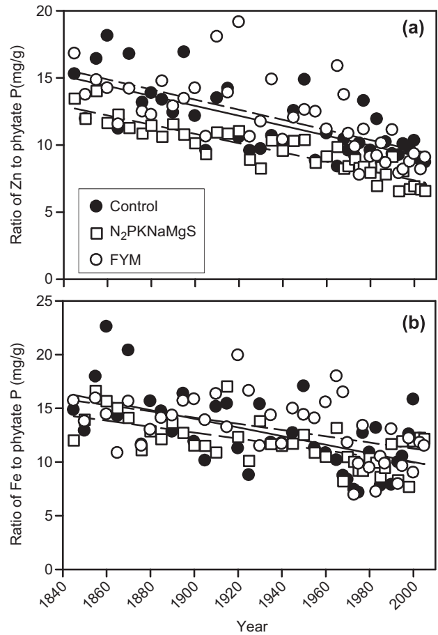
Fig. 2. The ratio of Zn (a) or Fe (b) to phytate P in wheat grain from three plots of the Broadbalk Experiment since 1845. Lines represent regression lines: dashed line for the control, dotted line for N 2 PKNaMgS, and solid line for FYM.
