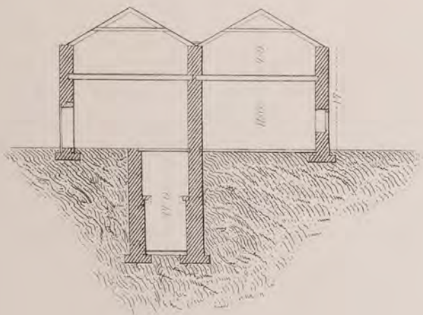
SECTION E.F.
