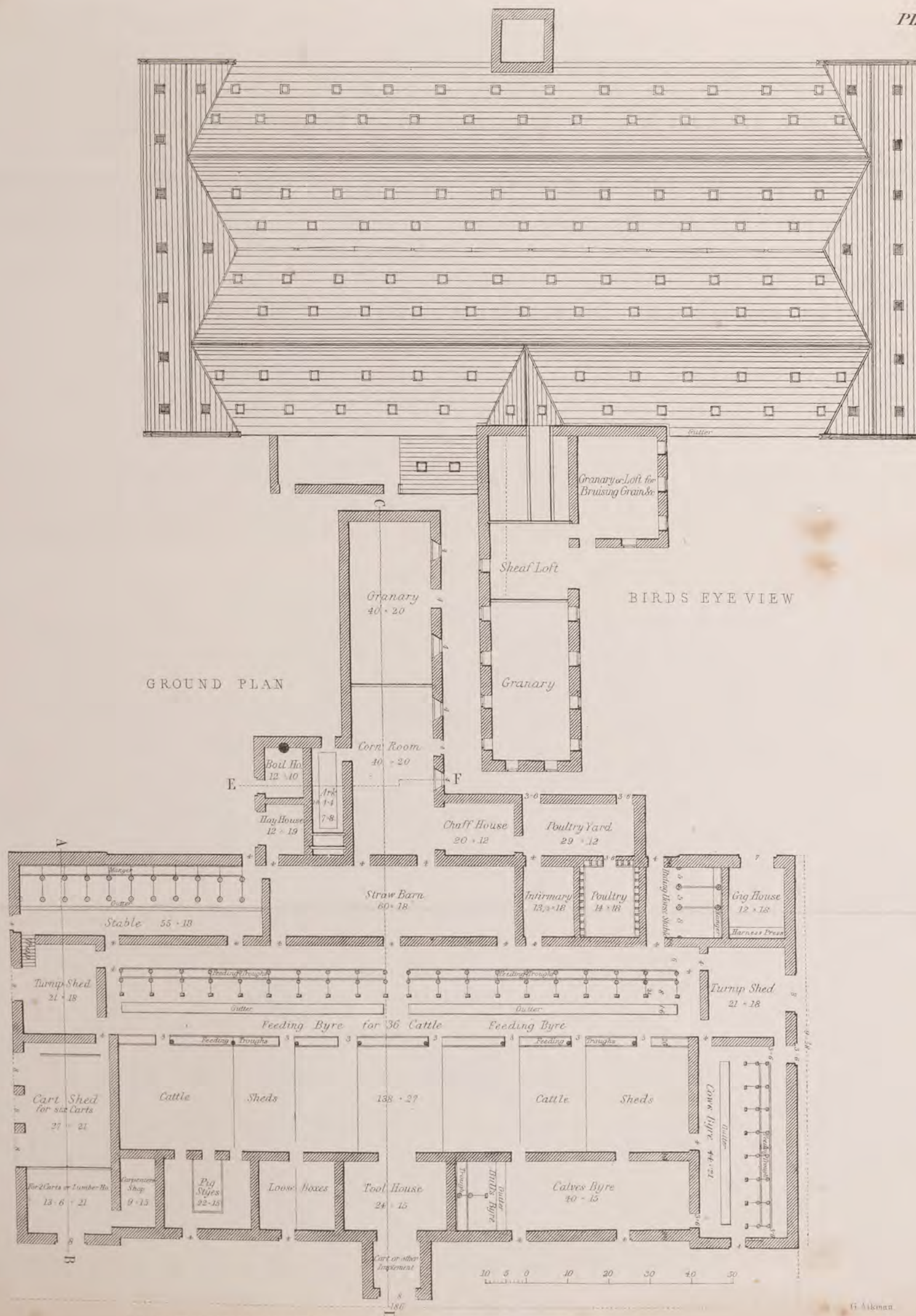
PLAN OF COVERED HOMESTEAD FOR A FARM OF 400 ACRES BY M r J. COWIE.
